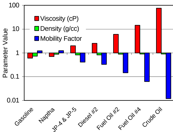
Figure 3-23c. Effective mobility of various LNAPL grades versus pure water with a mobility factor of 1.0. Notice that all other things being equal, viscosity plays the greatest role in changing pure phase mobility (where saturation is 100%).
