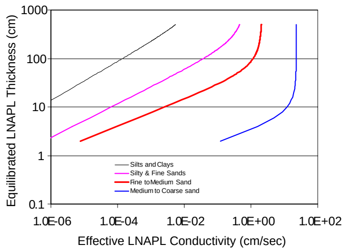
Figure 3-22. Effective LNAPL conductivity for JP-5 in different soils and under a range of observed thickness conditions.
