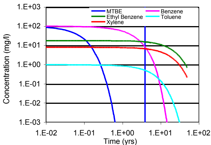
Figure 6-37. Hypothetical LNAPL zone depletion of soluble compound for conditions of a discrete LNAPL interval in only the sandy zone.
