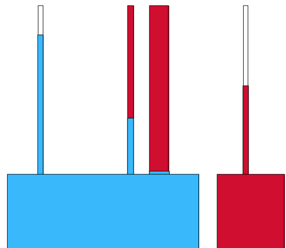
Figure 3-2. Capillary bath for 3 fluid phase couplets, water in blue, oil in red, air in white.
