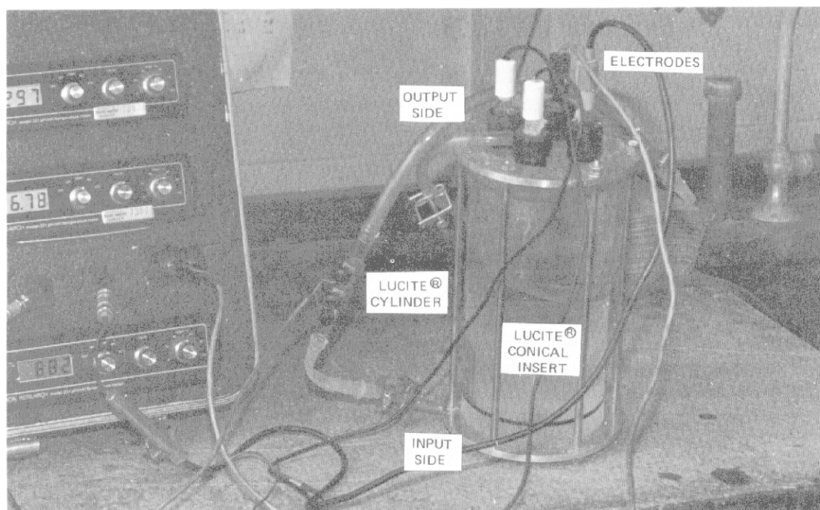
Figure 2.17. A well-head instrumentation package for Eh, pH, conductivity and temperature measurements
